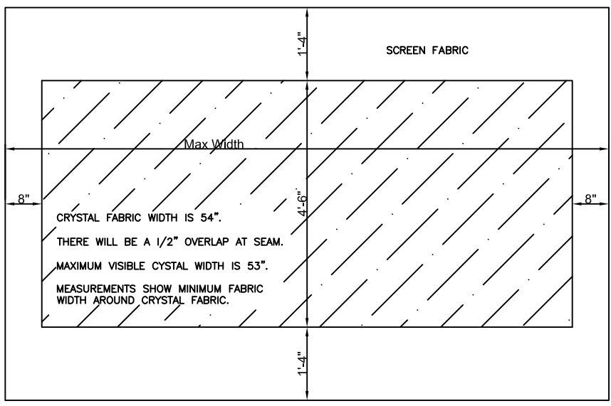
ROLLAC ZIPSHADE 150 SYSTEM SPECIFICATION WITH CRYSTAL FABRIC INSERT FOR VISIBILITY.
